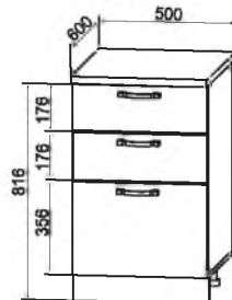
СЯБ 500 500/816/600
