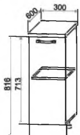
С 300 300/816/600
